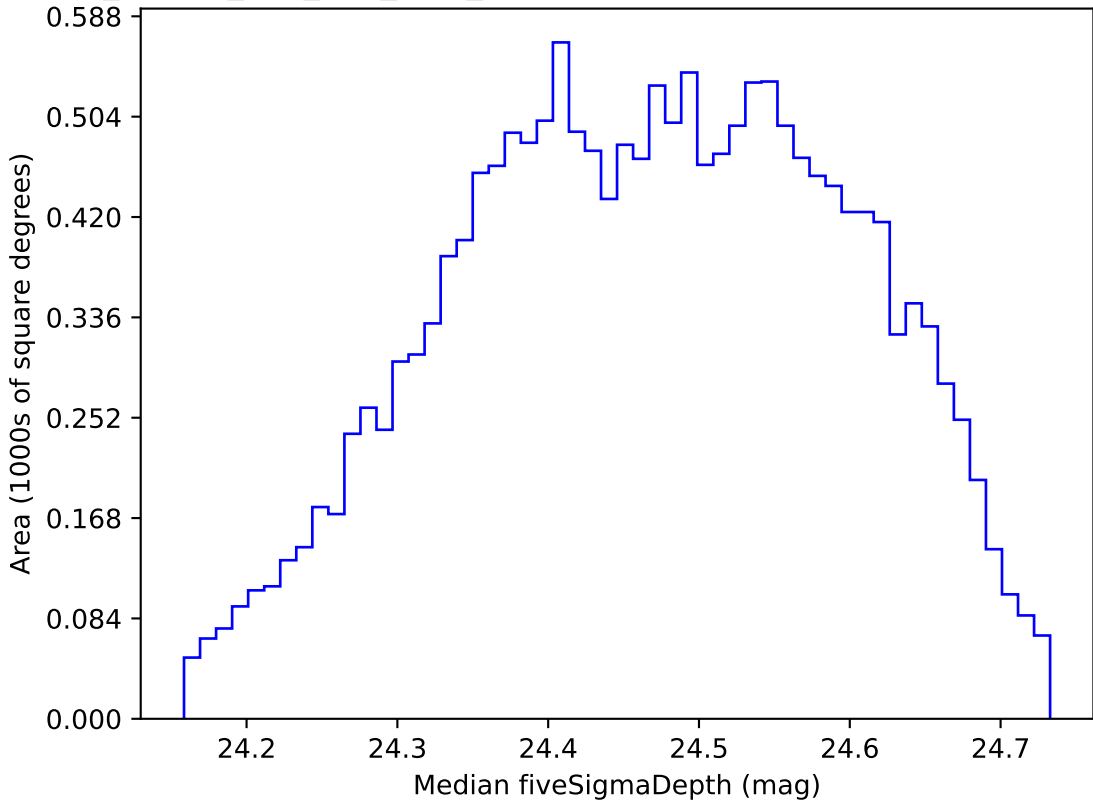
ddf_loaded_half_fl15_v3.4_10yrs WFD g band: Median fiveSigmaDepth
