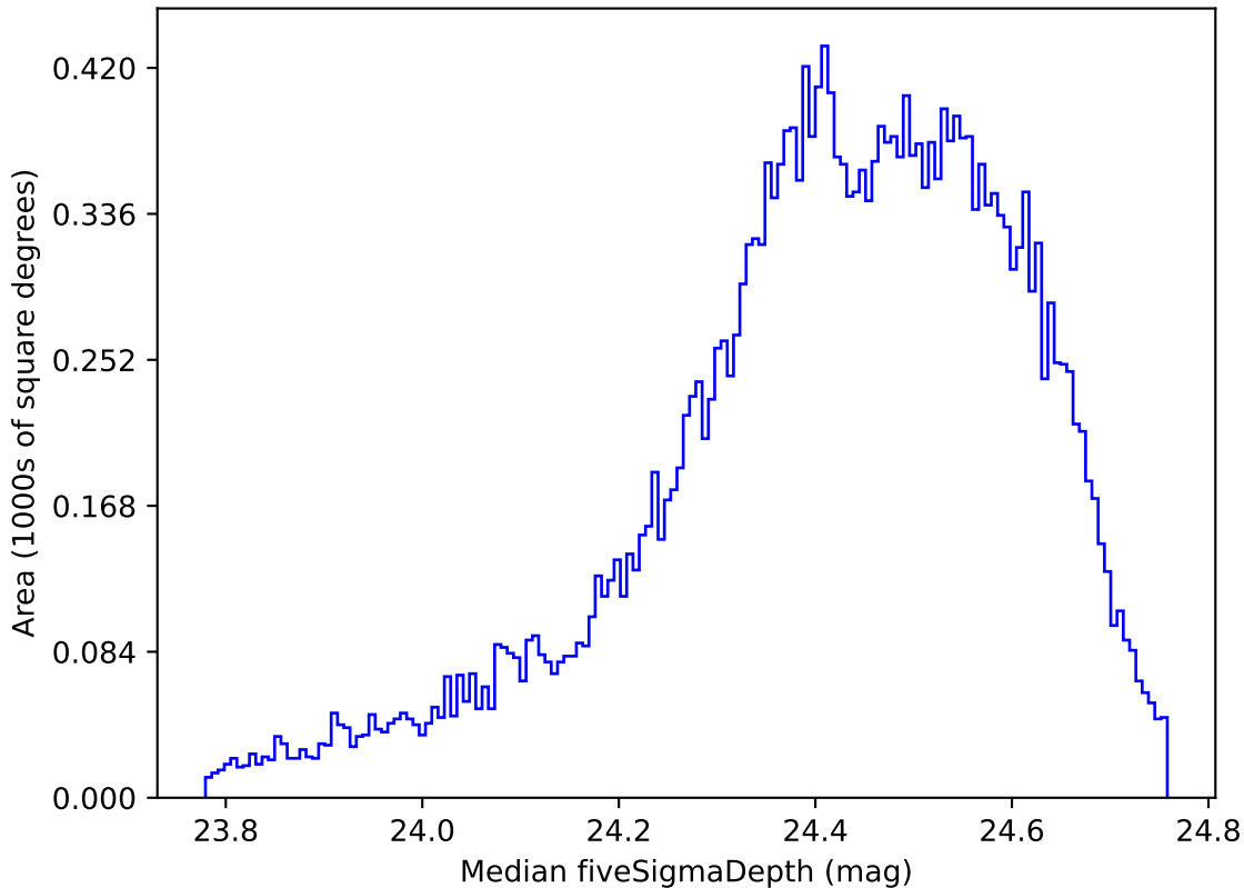
ddf_loaded_half_fl15_v3.4_10yrs All sky g band: Median fiveSigmaDepth
