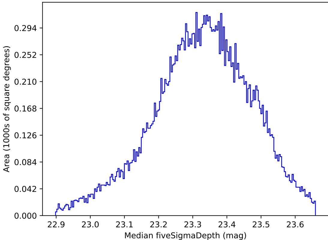
ddf_loaded_half_fl15_v3.4_10yrs All sky all bands: Median fiveSigmaDepth
