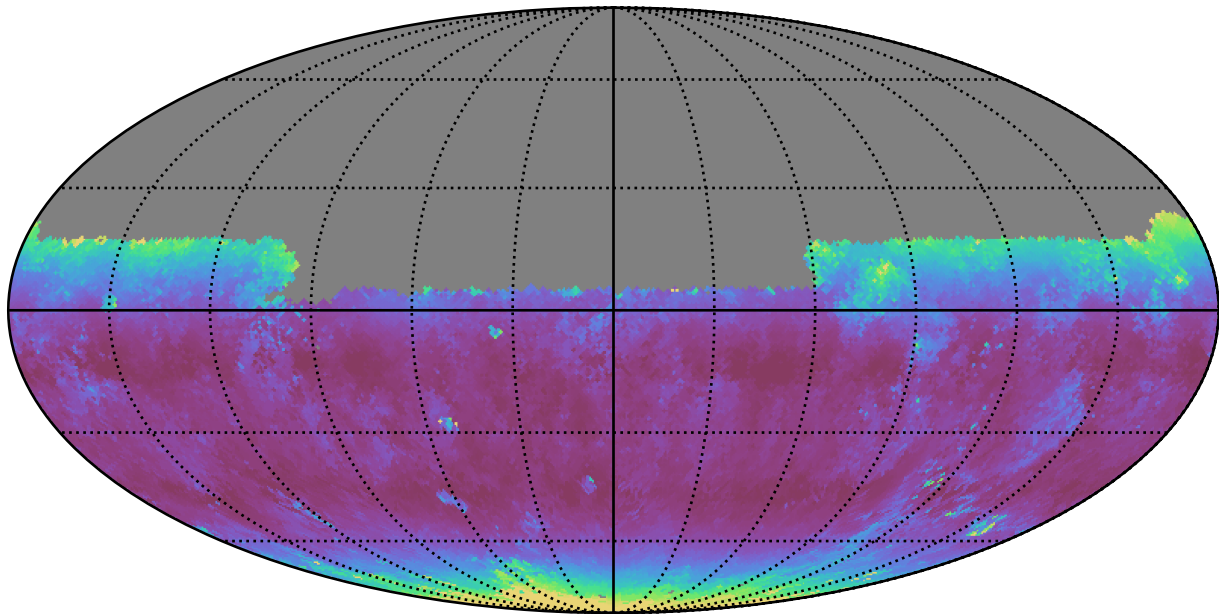
ddf_loaded_half_fl15_v3.4_10yrs Yr 1 y band: Median airmass
