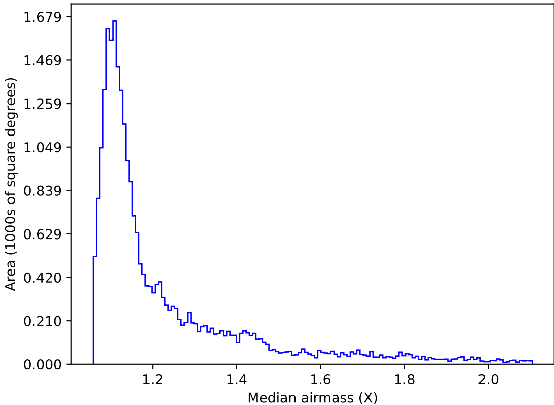
ddf_loaded_half_fl15_v3.4_10yrs Yr 1 i band: Median airmass
