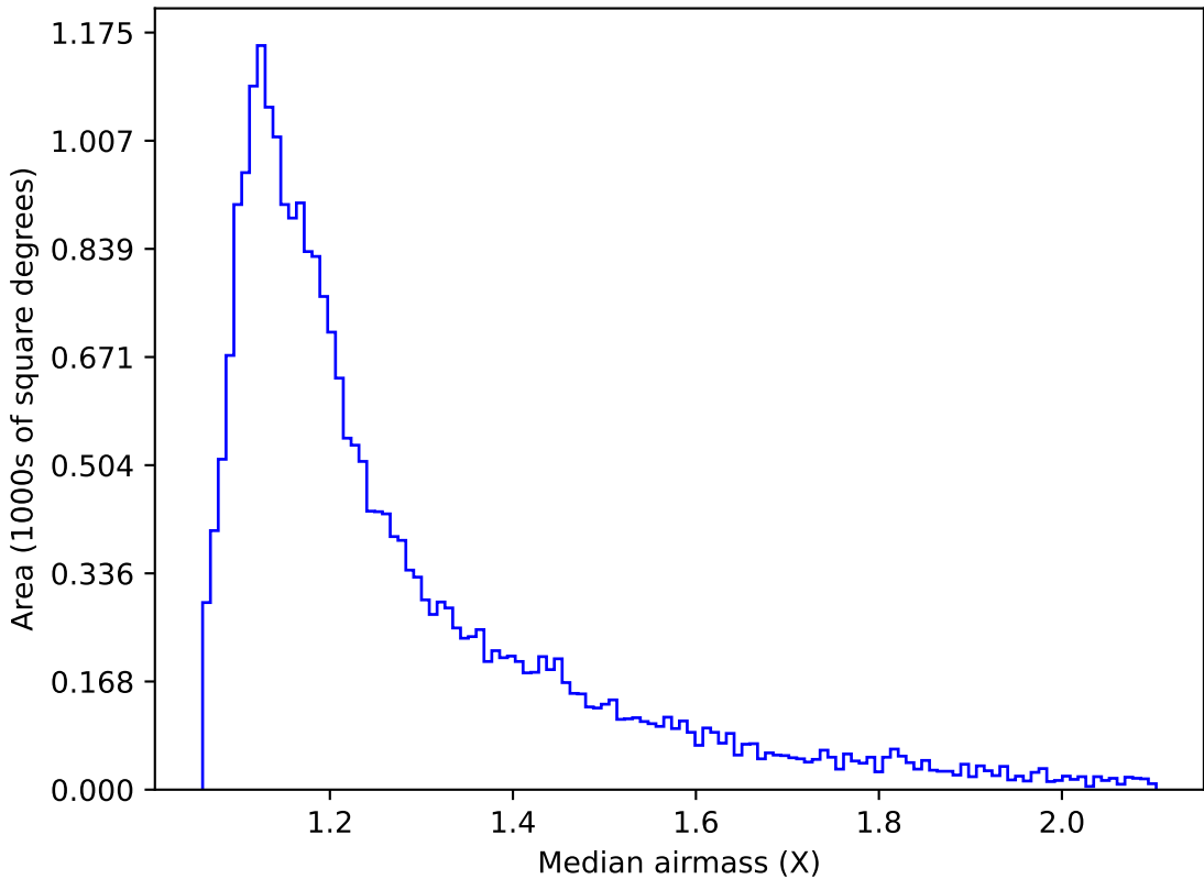
ddf_loaded_half_fl15_v3.4_10yrs Yr 1 g band: Median airmass
