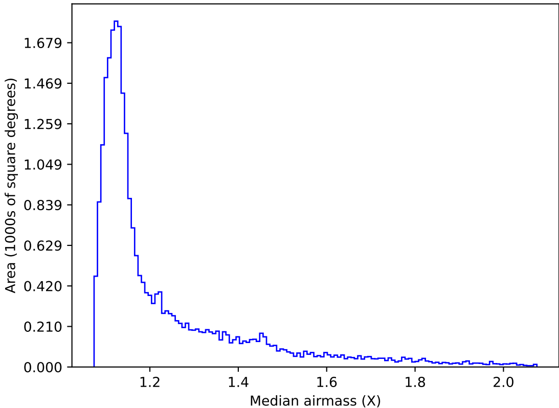
ddf_loaded_half_fl15_v3.4_10yrs Yr 1 all bands: Median airmass
