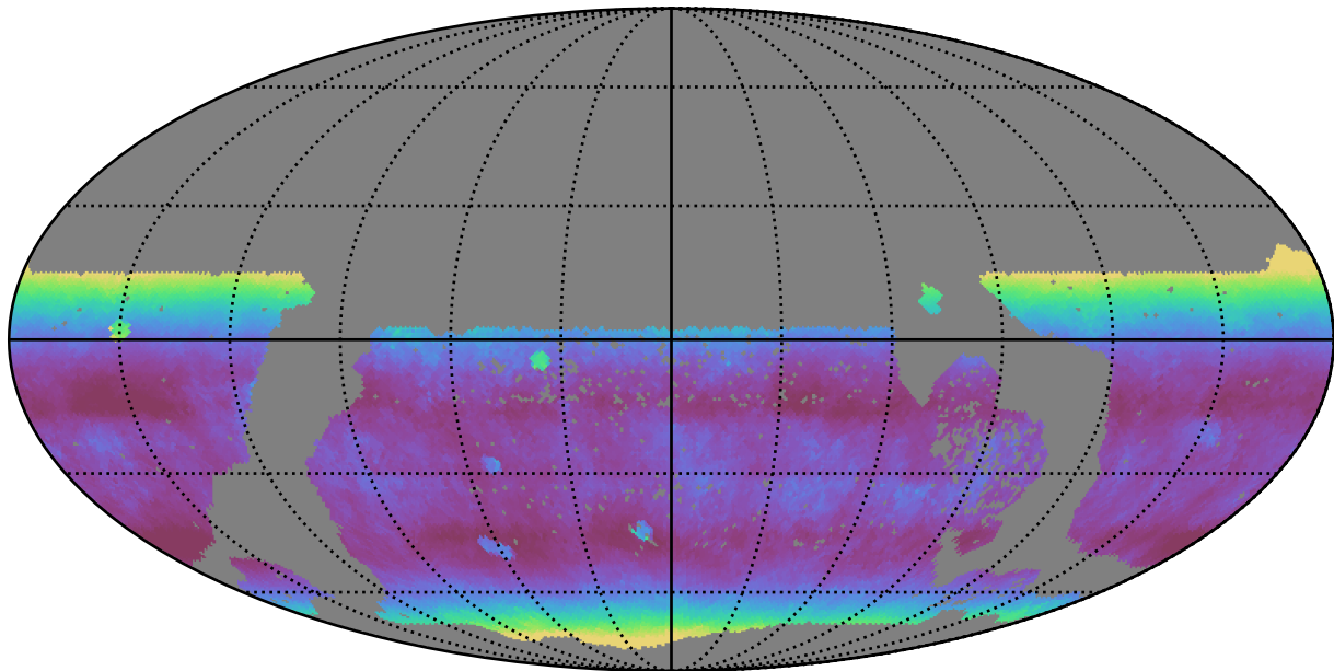
ddf_loaded_half_fl15_v3.4_10yrs WFD z band: Median airmass
