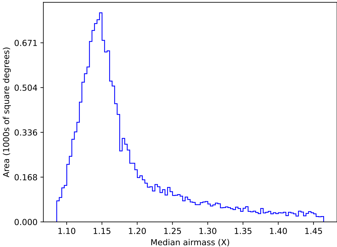
ddf_loaded_half_fl15_v3.4_10yrs WFD z band: Median airmass
