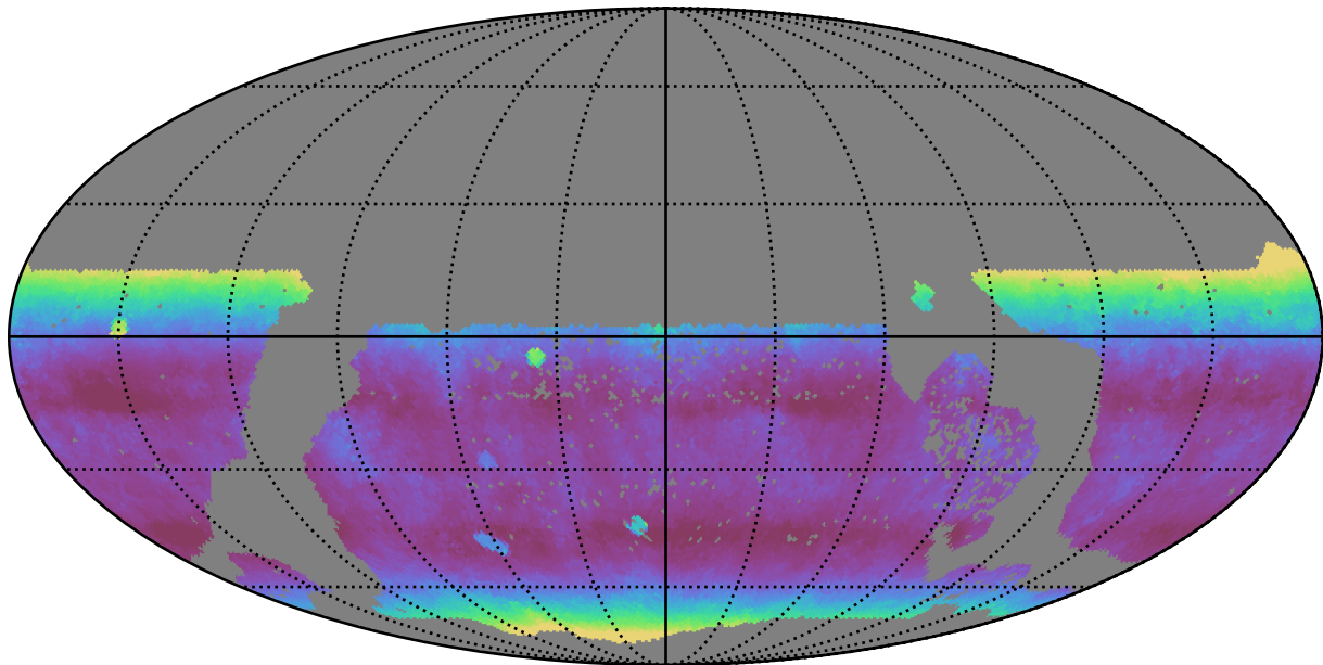
ddf_loaded_half_fl15_v3.4_10yrs WFD y band: Median airmass
