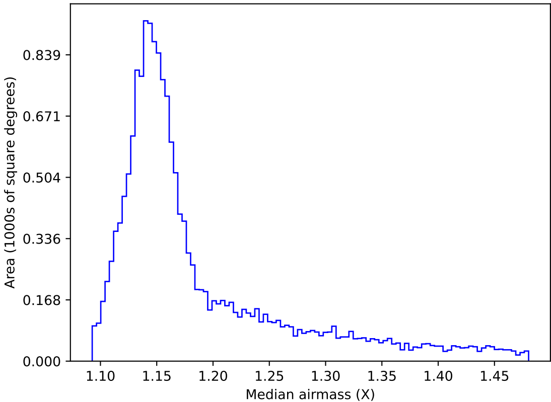
ddf_loaded_half_fl15_v3.4_10yrs WFD y band: Median airmass
