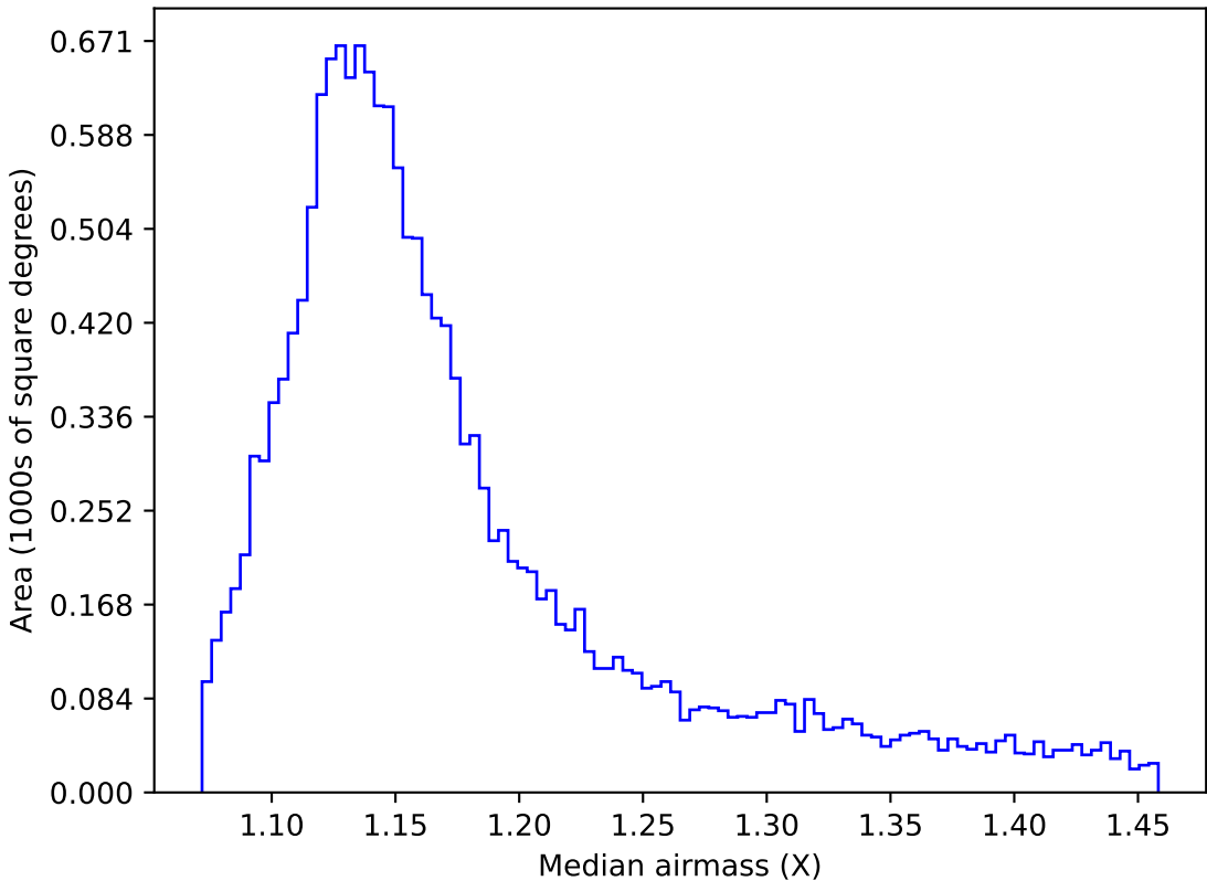
ddf_loaded_half_fl15_v3.4_10yrs WFD u band: Median airmass
