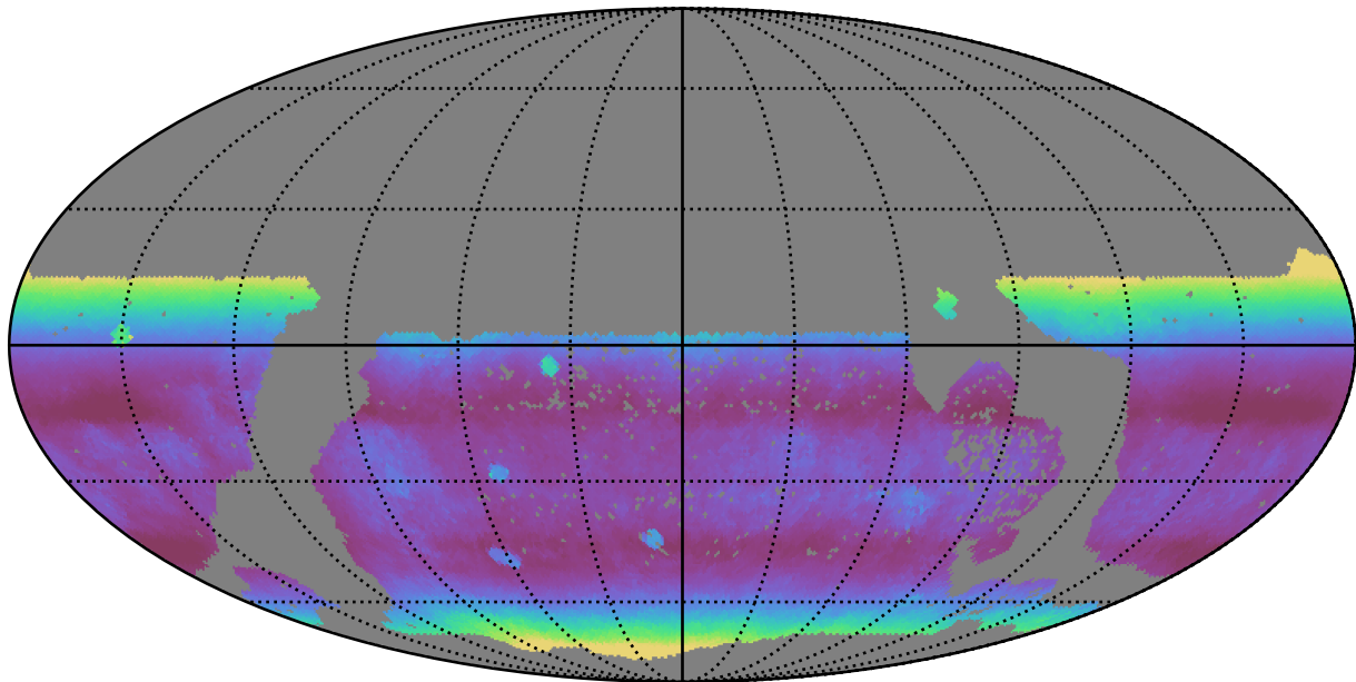
ddf_loaded_half_fl15_v3.4_10yrs WFD r band: Median airmass
