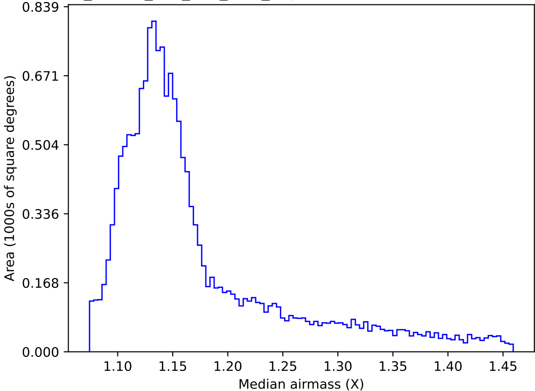
ddf_loaded_half_fl15_v3.4_10yrs WFD r band: Median airmass
