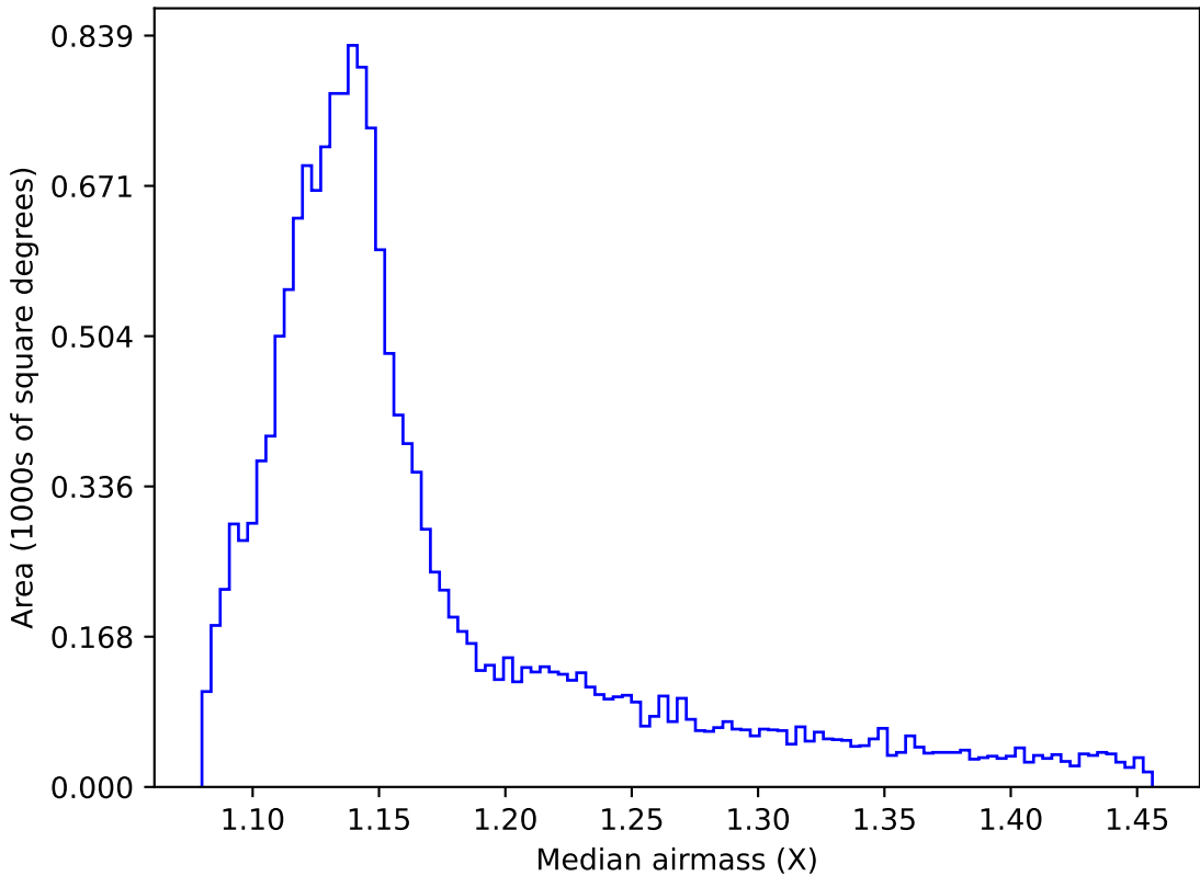
ddf_loaded_half_fl15_v3.4_10yrs WFD i band: Median airmass
