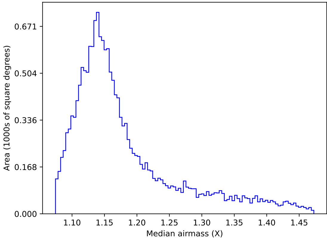
ddf_loaded_half_fl15_v3.4_10yrs WFD g band: Median airmass
