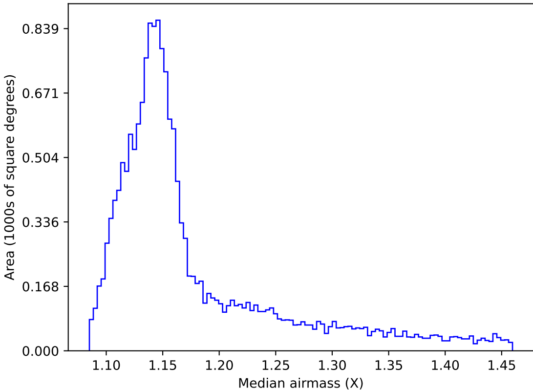
ddf_loaded_half_fl15_v3.4_10yrs WFD all bands: Median airmass
