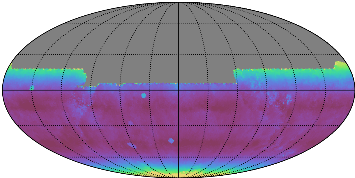
ddf_loaded_half_fl15_v3.4_10yrs All sky y band: Median airmass
