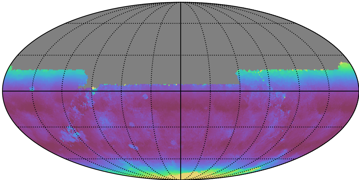
ddf_loaded_half_fl15_v3.4_10yrs All sky u band: Median airmass
