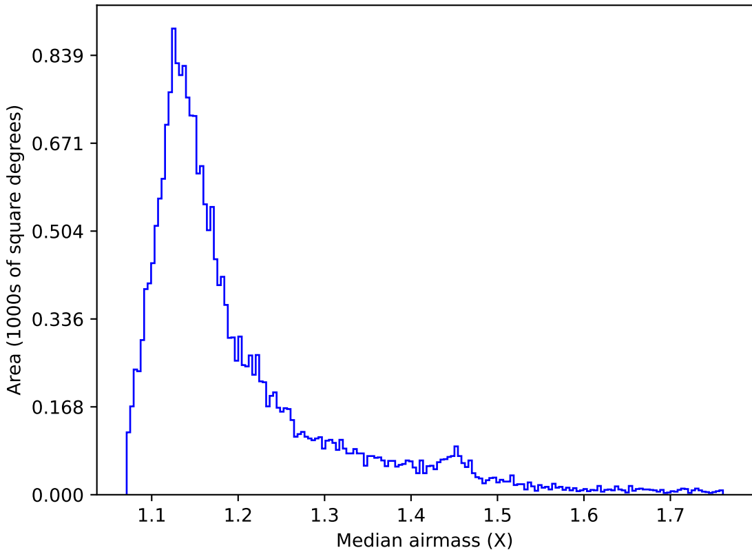
ddf_loaded_half_fl15_v3.4_10yrs All sky u band: Median airmass
