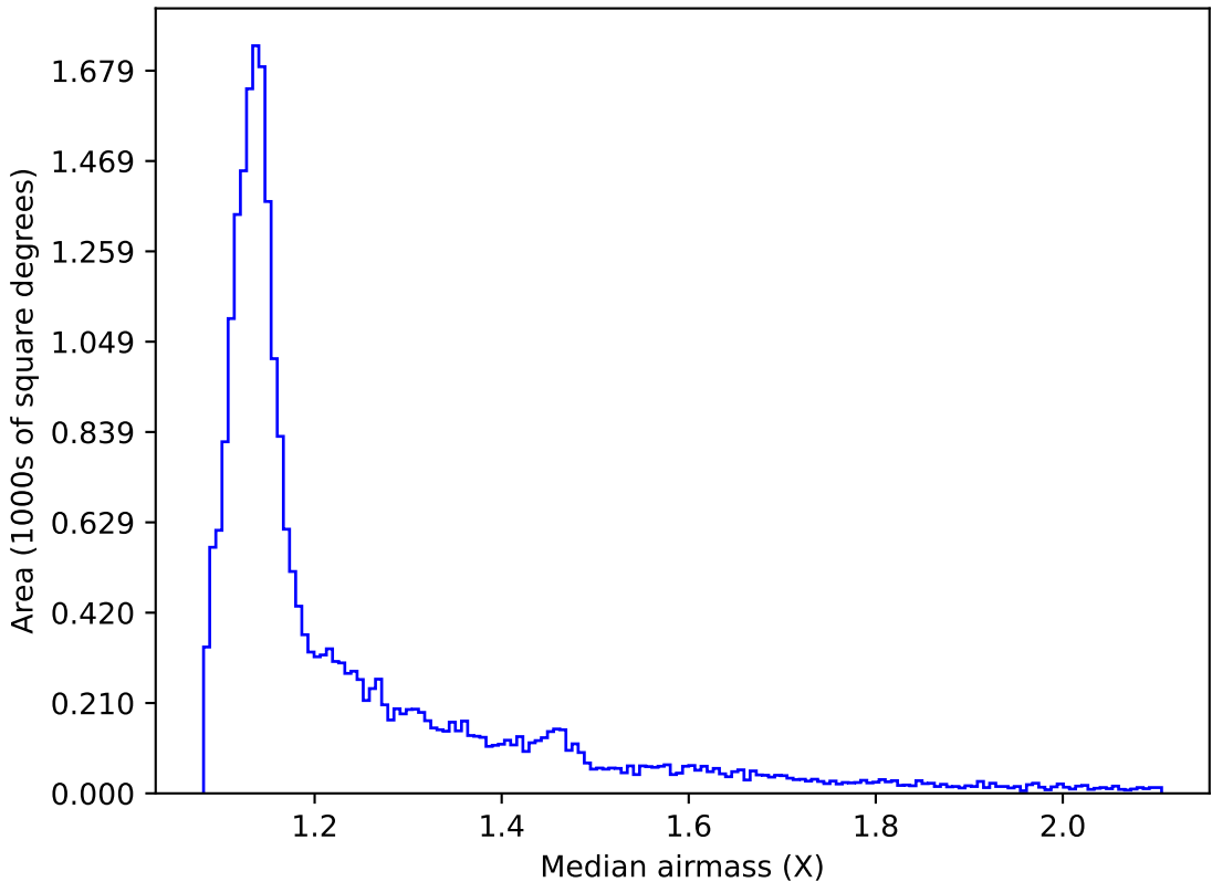
ddf_loaded_half_fl15_v3.4_10yrs All sky i band: Median airmass
