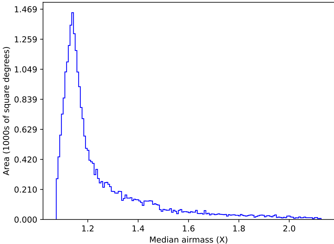
ddf_loaded_half_fl15_v3.4_10yrs All sky g band: Median airmass
