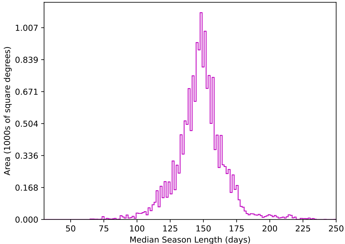
ddf_loaded_half_fl15_v3.4_10yrs WFD z band: Median Season Length
