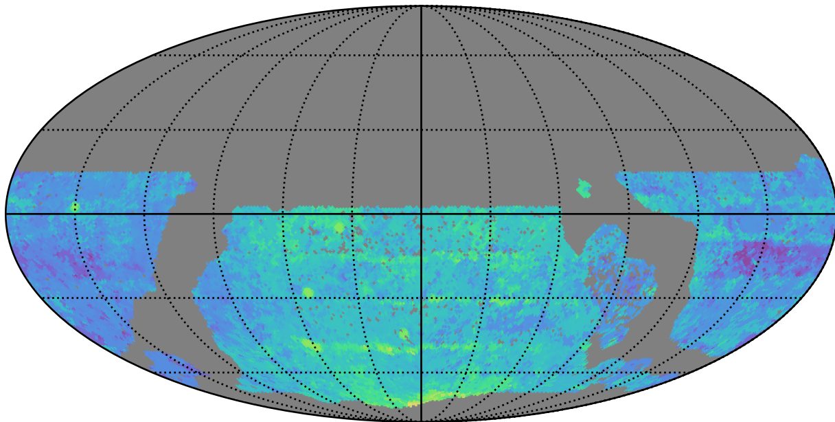
ddf_loaded_half_fl15_v3.4_10yrs WFD y band: Median Season Length
