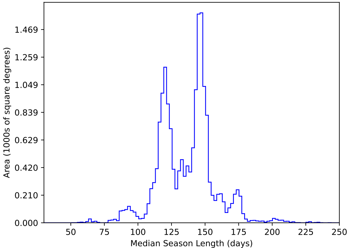
ddf_loaded_half_fl15_v3.4_10yrs WFD y band: Median Season Length
