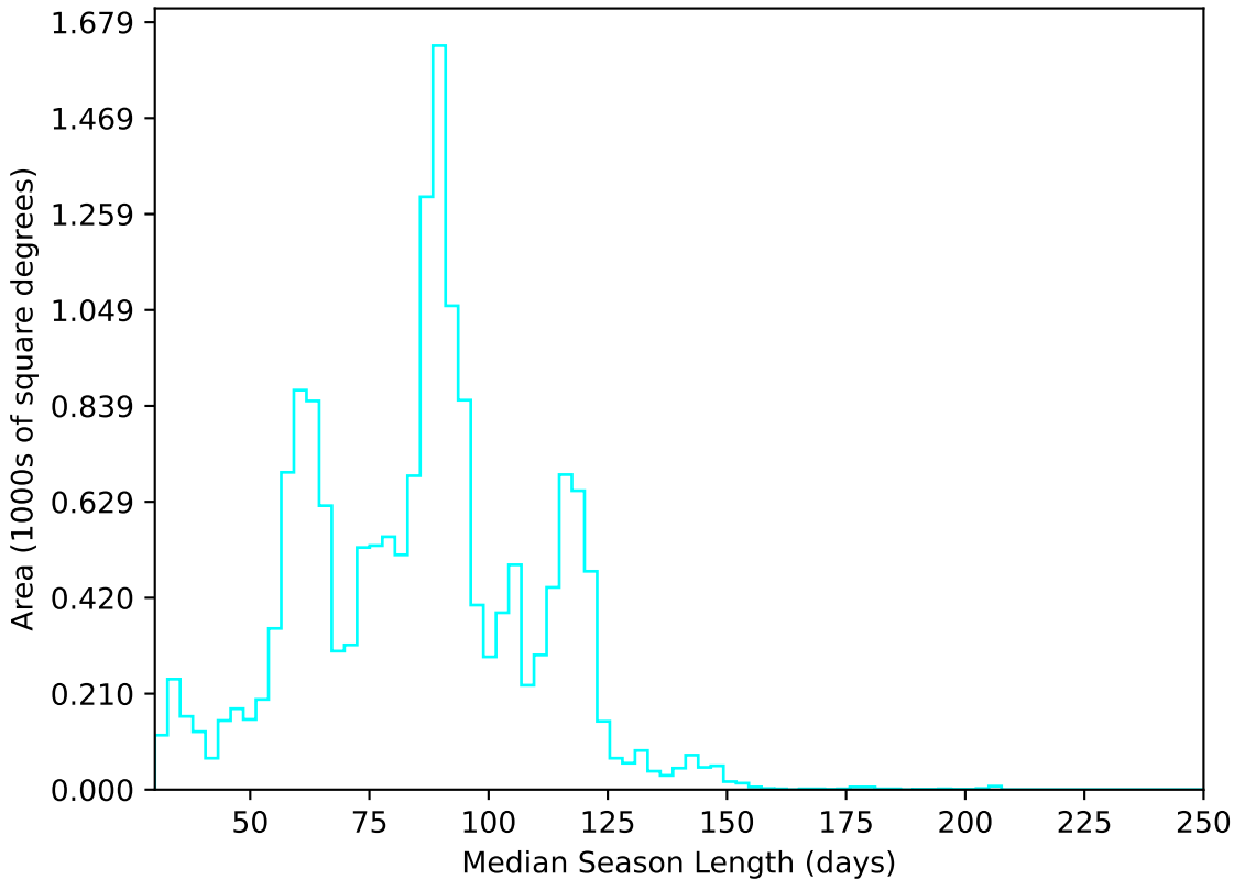
ddf_loaded_half_fl15_v3.4_10yrs WFD u band: Median Season Length
