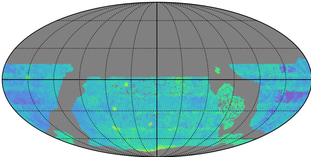
ddf_loaded_half_fl15_v3.4_10yrs WFD i band: Median Season Length
