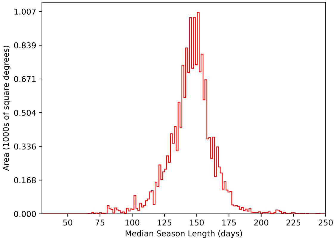
ddf_loaded_half_fl15_v3.4_10yrs WFD i band: Median Season Length
