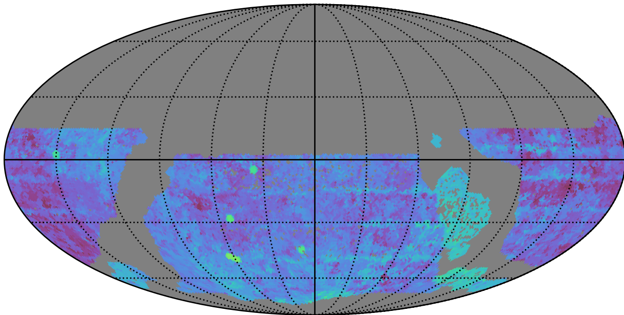
ddf_loaded_half_fl15_v3.4_10yrs WFD g band: Median Season Length
