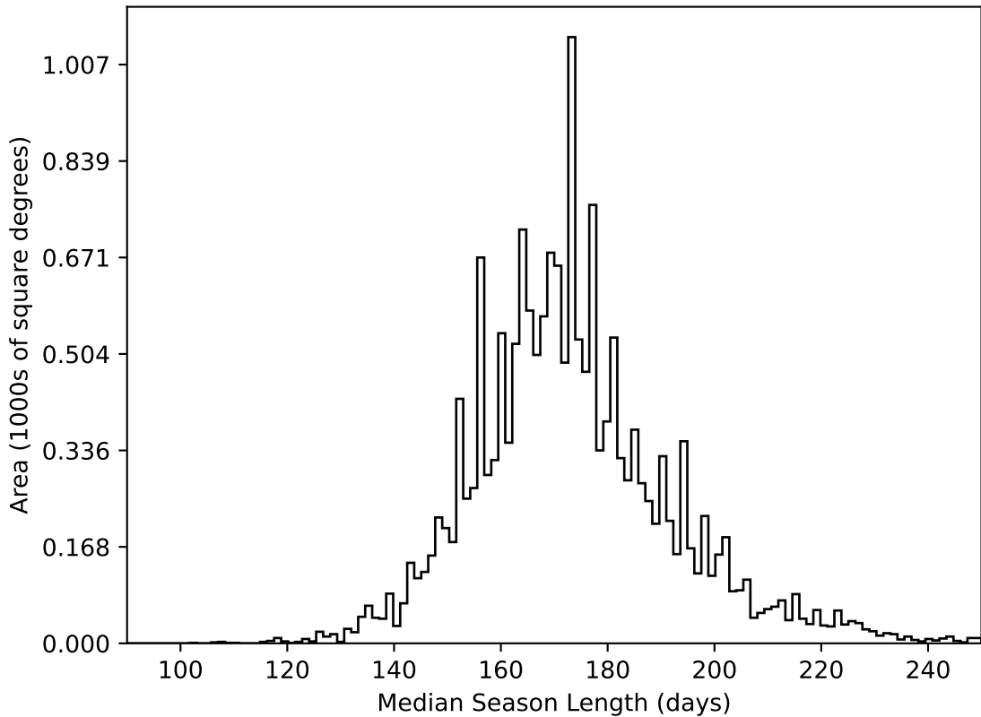
ddf_loaded_half_fl15_v3.4_10yrs WFD all bands: Median Season Length
