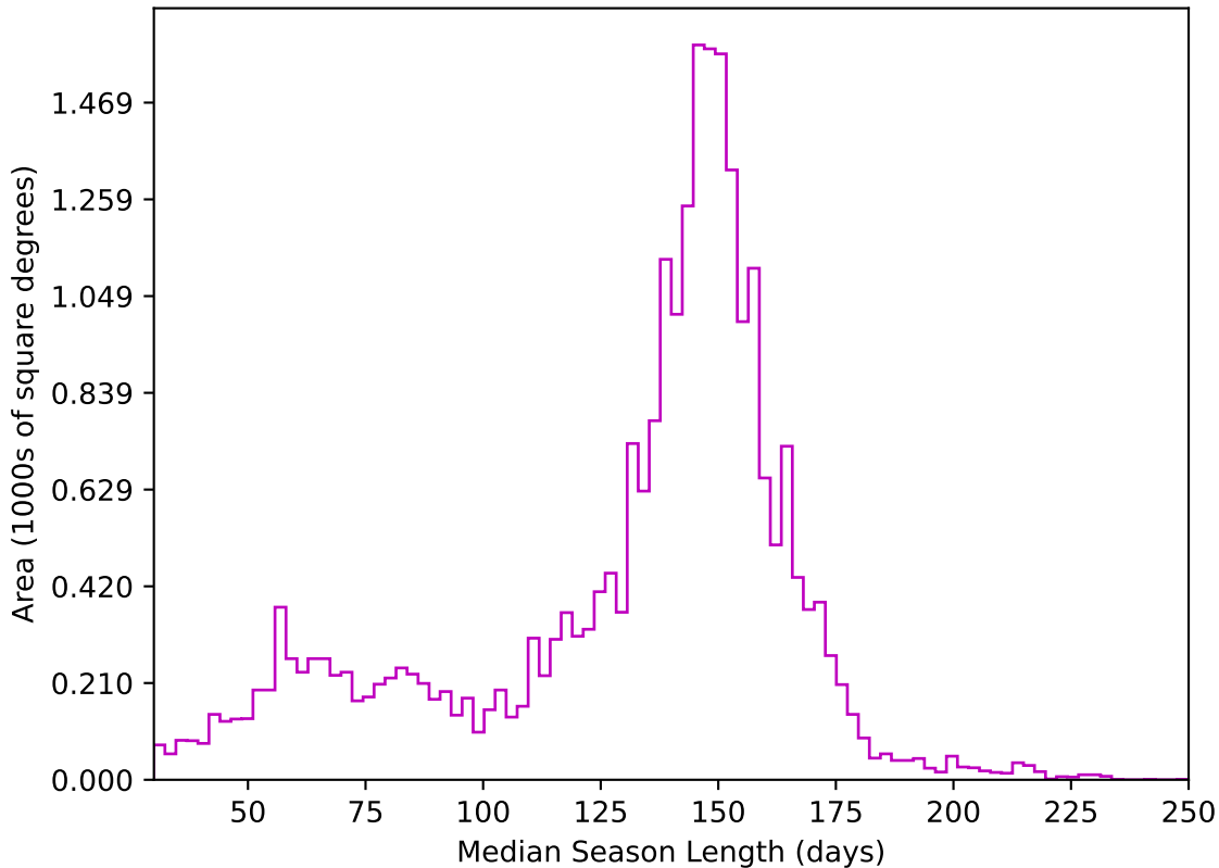
ddf_loaded_half_fl15_v3.4_10yrs All sky z band: Median Season Length
