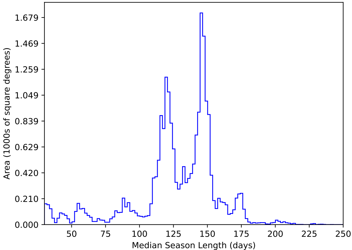
ddf_loaded_half_fl15_v3.4_10yrs All sky y band: Median Season Length
