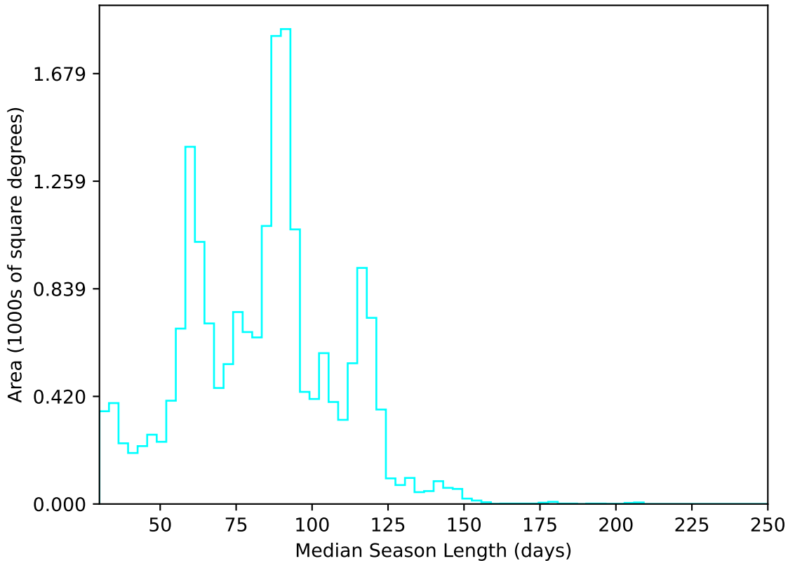
ddf_loaded_half_fl15_v3.4_10yrs All sky u band: Median Season Length
