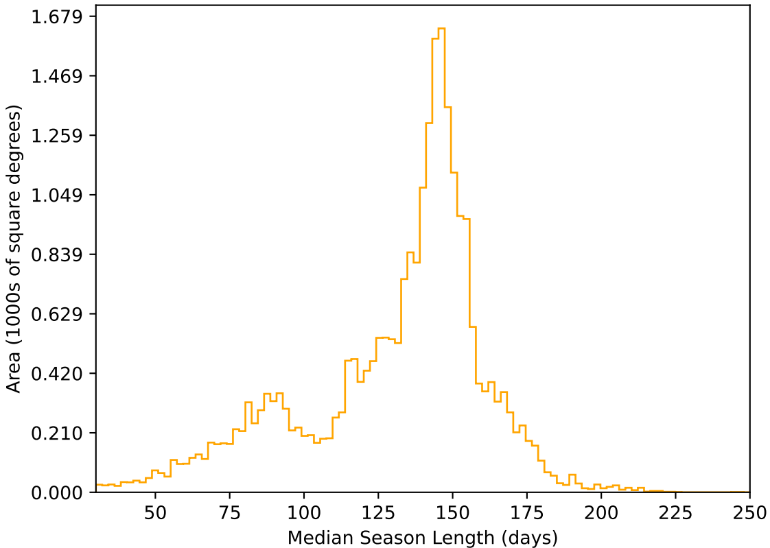
ddf_loaded_half_fl15_v3.4_10yrs All sky r band: Median Season Length
