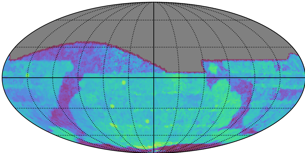
ddf_loaded_half_fl15_v3.4_10yrs All sky i band: Median Season Length
