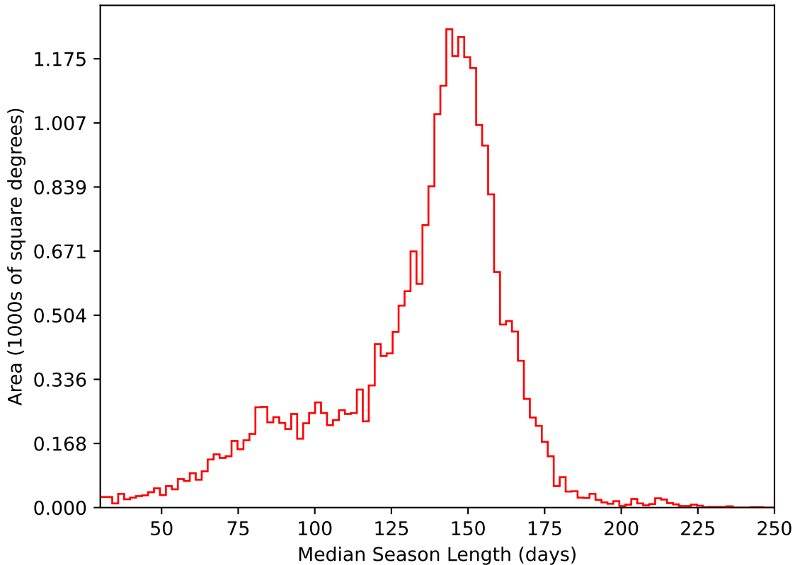
ddf_loaded_half_fl15_v3.4_10yrs All sky i band: Median Season Length
