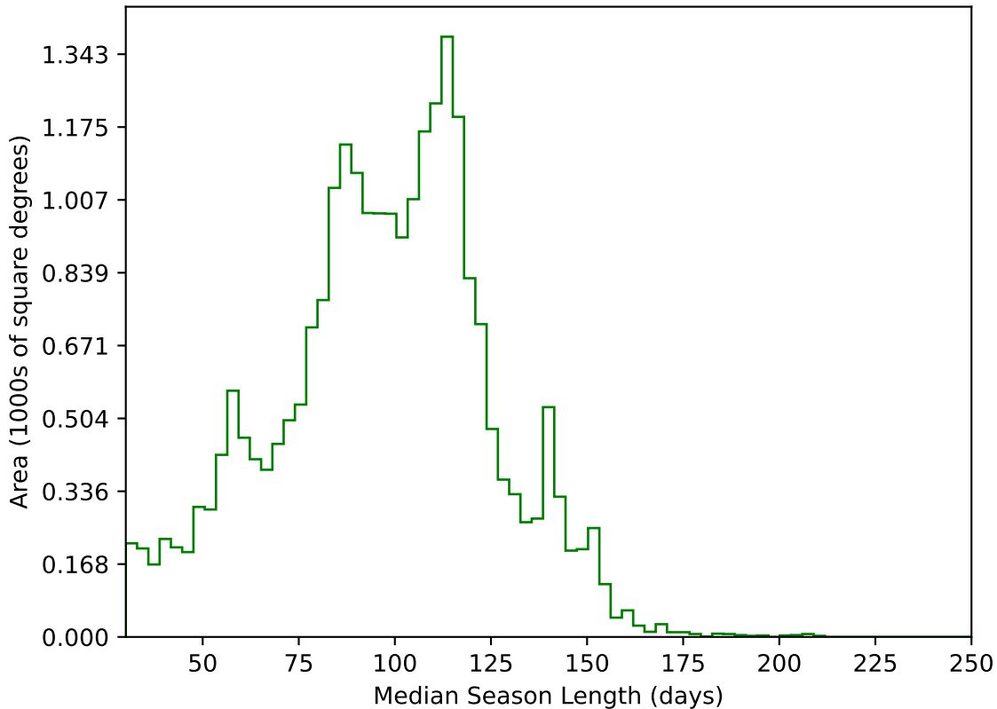
ddf_loaded_half_fl15_v3.4_10yrs All sky g band: Median Season Length
