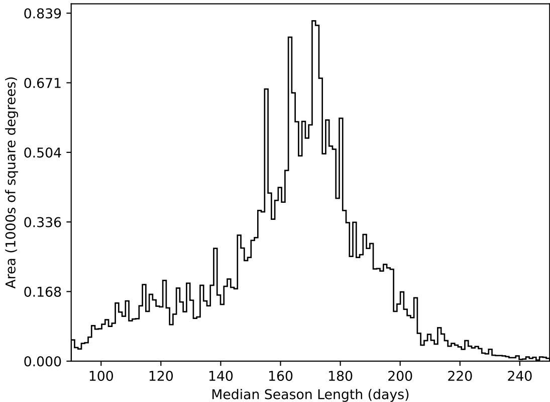
ddf_loaded_half_fl15_v3.4_10yrs All sky all bands: Median Season Length
