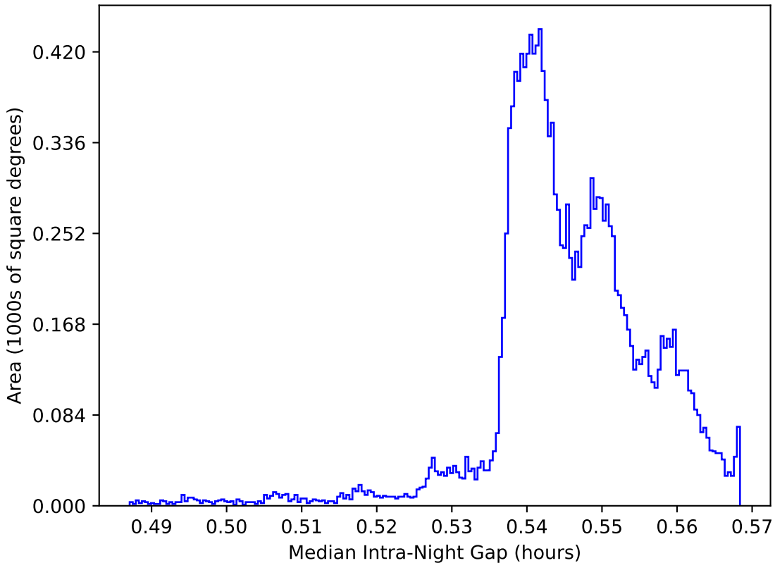
ddf_loaded_half_fl15_v3.4_10yrs WFD: Median Intra-Night Gap
