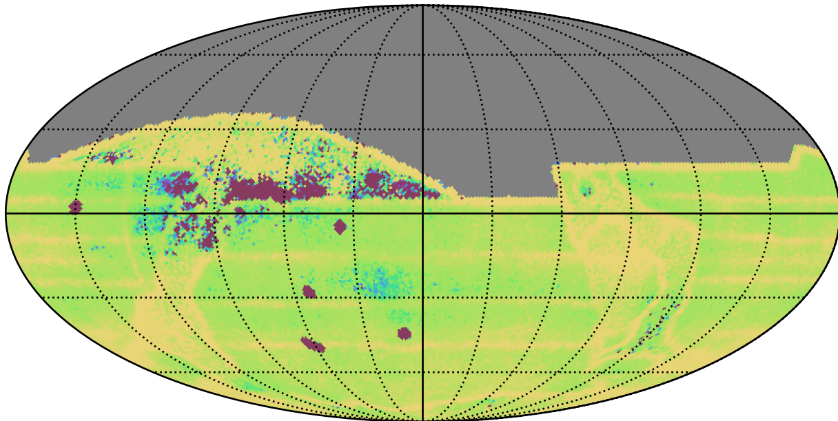
ddf_loaded_half_fl15_v3.4_10yrs All sky: Median Intra-Night Gap
