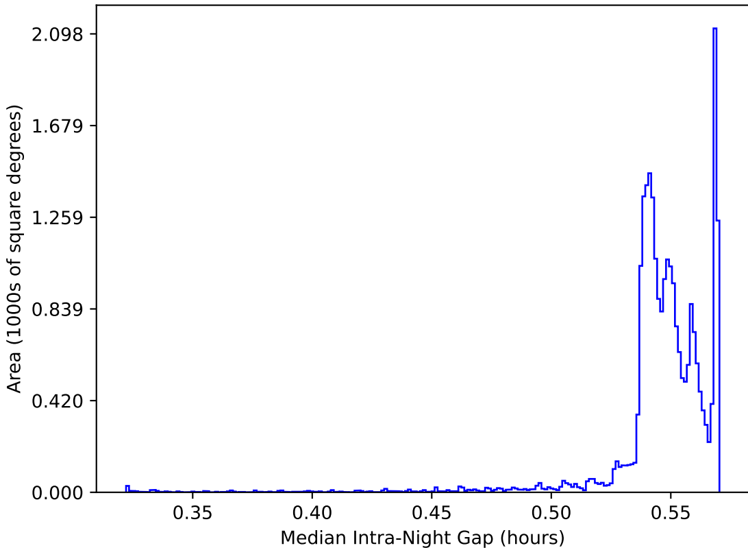
ddf_loaded_half_fl15_v3.4_10yrs All sky: Median Intra-Night Gap
