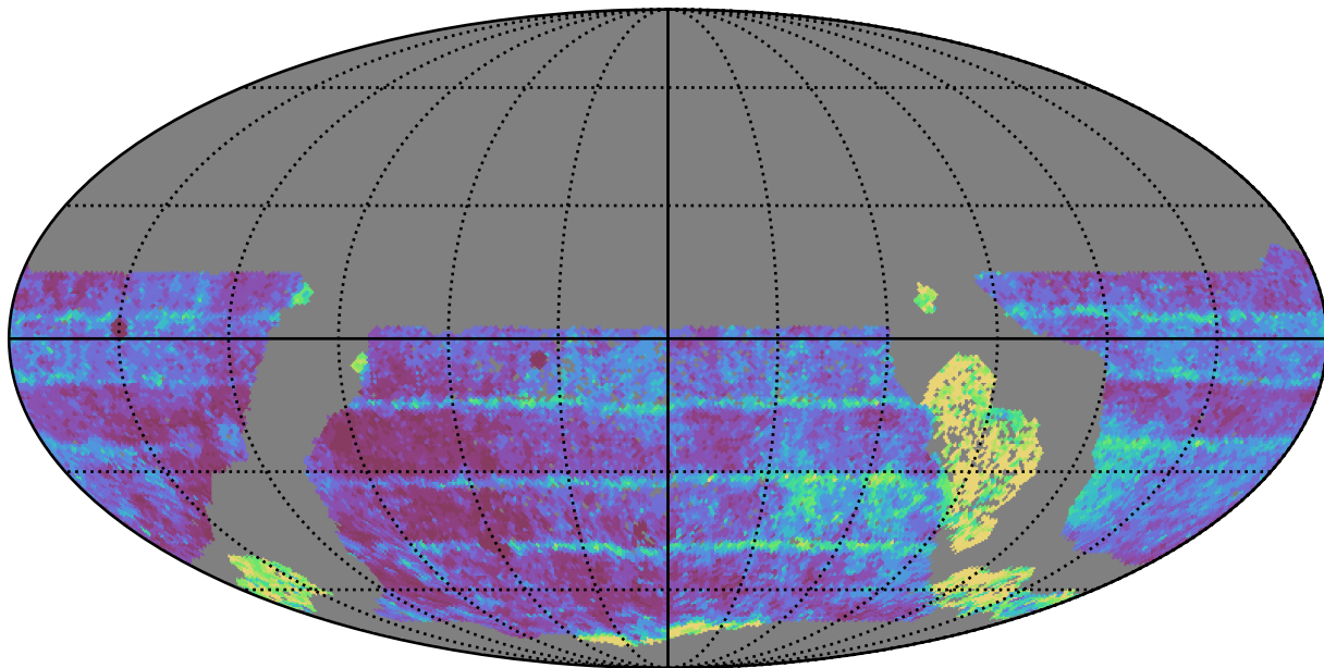
ddf_loaded_half_fl15_v3.4_10yrs WFD z band: Median Inter-Night Gap
