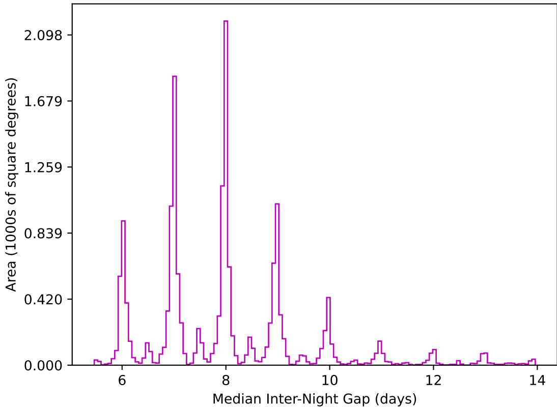
ddf_loaded_half_fl15_v3.4_10yrs WFD z band: Median Inter-Night Gap
