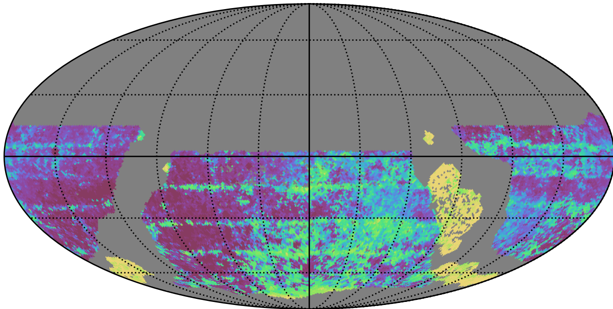
ddf_loaded_half_fl15_v3.4_10yrs WFD y band: Median Inter-Night Gap
