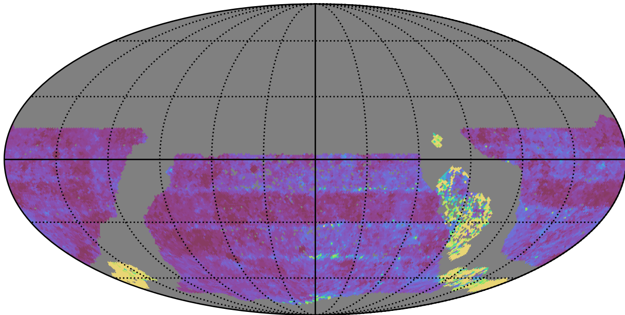
ddf_loaded_half_fl15_v3.4_10yrs WFD u band: Median Inter-Night Gap
