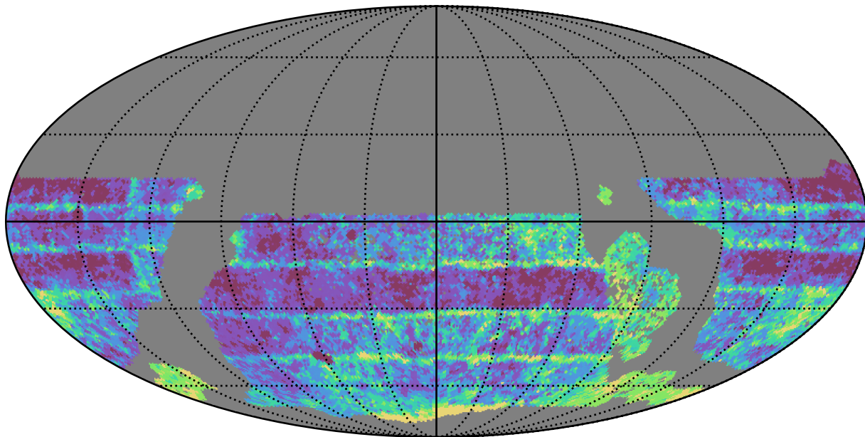
ddf_loaded_half_fl15_v3.4_10yrs WFD r band: Median Inter-Night Gap
