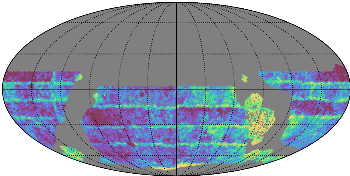
ddf_loaded_half_fl15_v3.4_10yrs WFD i band: Median Inter-Night Gap
