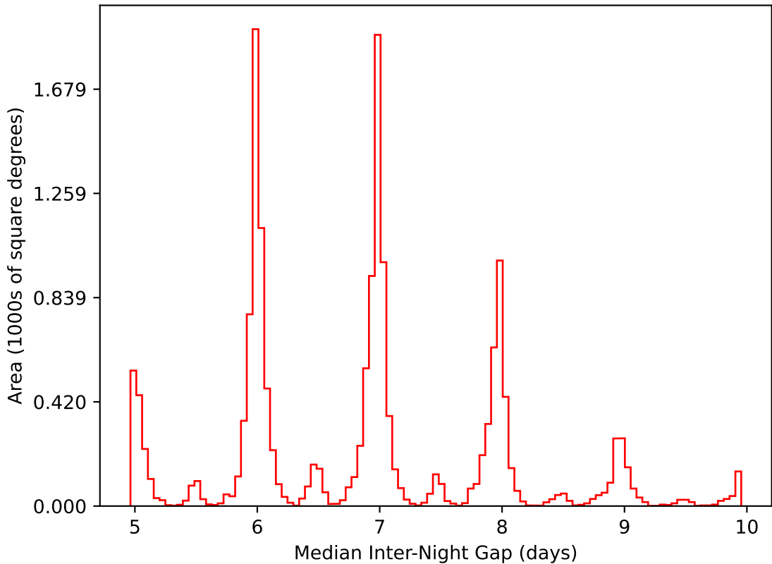
ddf_loaded_half_fl15_v3.4_10yrs WFD i band: Median Inter-Night Gap
