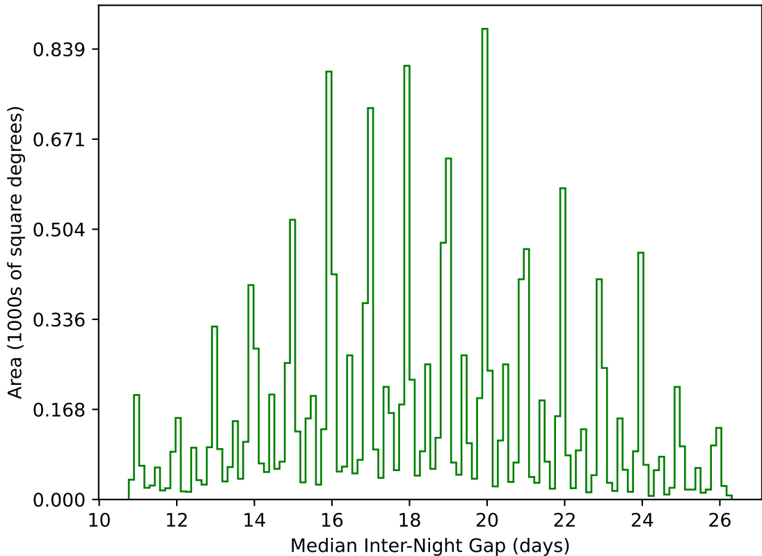
ddf_loaded_half_fl15_v3.4_10yrs WFD g band: Median Inter-Night Gap
