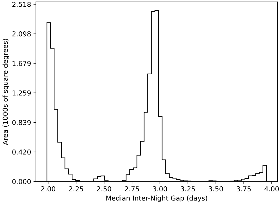
ddf_loaded_half_fl15_v3.4_10yrs WFD all bands: Median Inter-Night Gap
